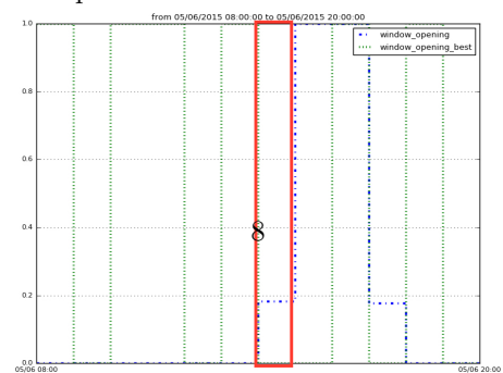
Figure 5: Actual and recommended door position
