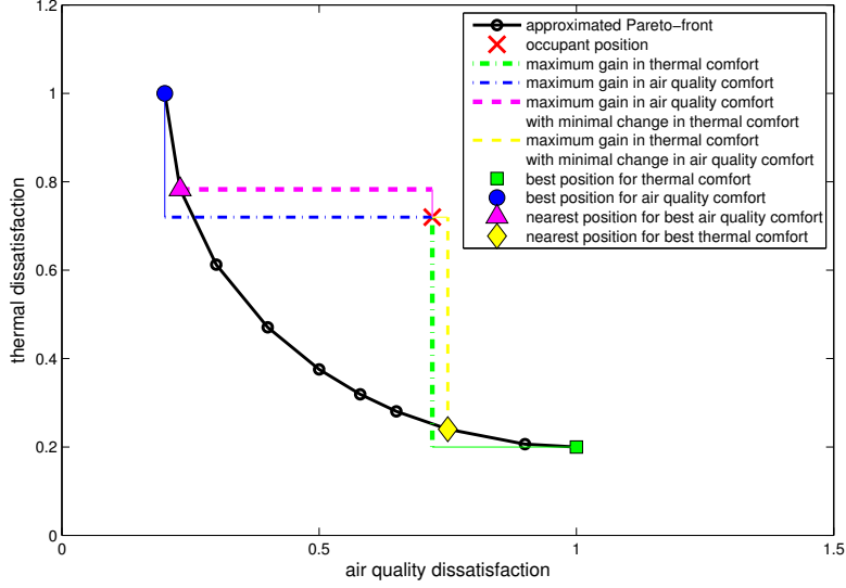
Figure 7: Optimal scenario and consequences of occupant’s historical actions.
