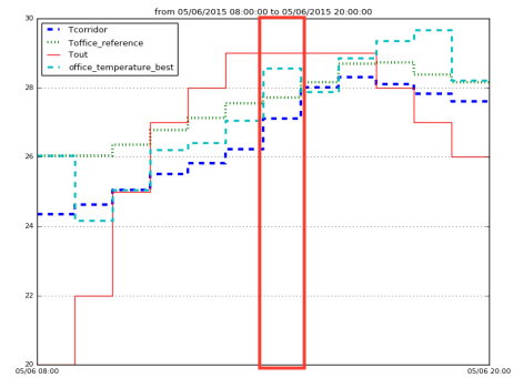
Figure 3: Different temperature measurements and system output
