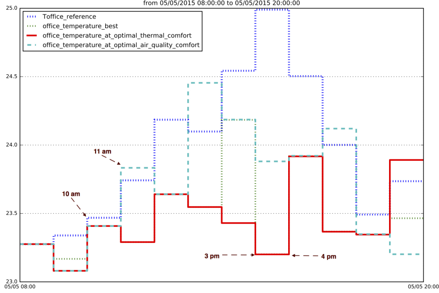
Figure 9: Average office temperatures at different hours showing the proposed temperatures and the recorded temperatures
