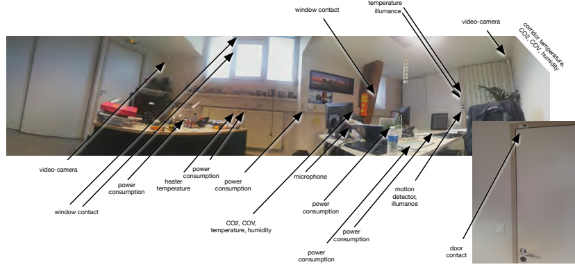
Figure 1: Panoramic photo of the office with sensors
