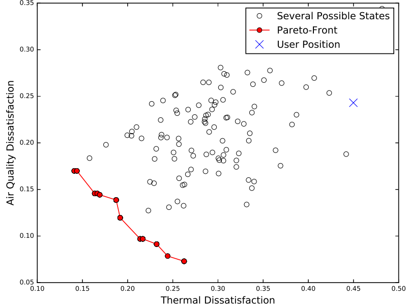
Figure 8: Results from Multi-objective Differential Evolution for comparison with User Position
