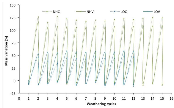
Fig. 10 : Mass evolution during drying/wetting cycles of weathering test with full immersion
