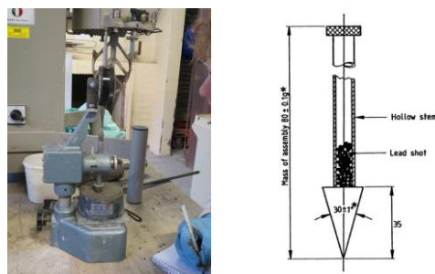
Fig. 1: Penetration test.
