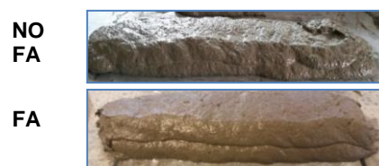
Fig. 6: Layers of 3 D printing with and without FA
