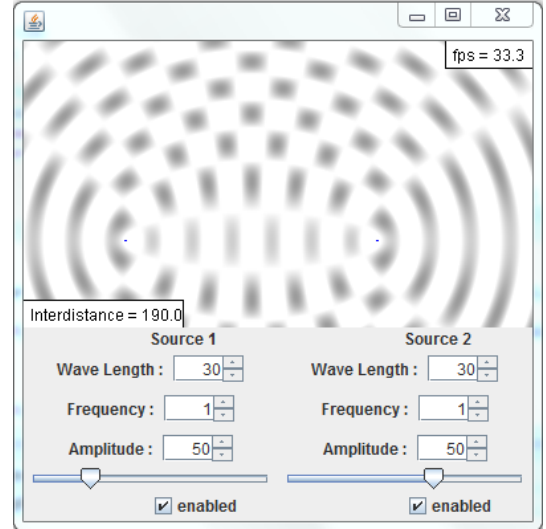
Fig. 3. Screen-shot of the experimental prototype of WAVE featuring the wave propagation model and using two emitter agents (black dots). The selected wave sources parameters generate distinct patterns called interference fringes.
