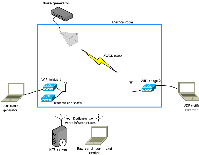
Fig. 1. Implementation of the wireless test bench.
