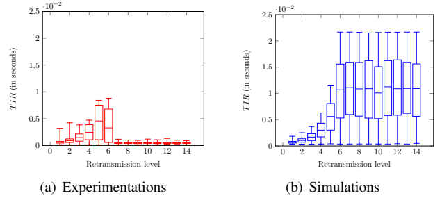
Fig. 9. TIR values measured on the experimentations 9(a) and simulation data 9(b). Values are presented with regards to the level of retransmission. For each trace, the figures depict the min, median and max values as well as the 1st and 3rd quartiles.
