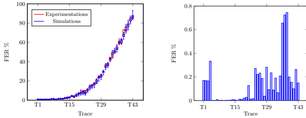
(a) Experimentations and simulations (b) Differences between paired FER FER after trace pairing
