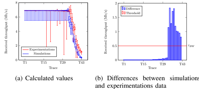
Fig. 7. Data for BW metric. Graph 7(a) shows the median, the 1st and 3rd quartile, as well as the min and max values for the BW metric measured on the simulation and experimentation traces. Graph 7(b) shows the differences measured for M(BW) between the paired traces of the simulation and the experimental datasets.
