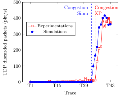
Fig. 8. Values of M(DROP) on the paired traces.
