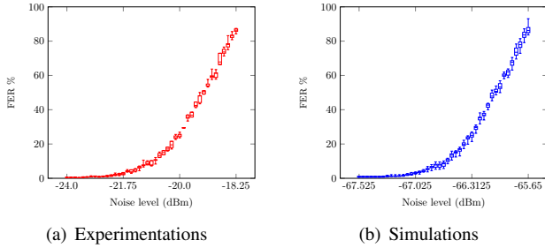
Fig. 2. FER measures regarding the different noise levels in experimentations 2(a) and simulations 2(b). The values are for each trace the 1st and 3rd quartile, as well as the min and max values. The central value displayed is the median.
