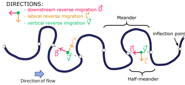
Fig. 8 Definition of the three migration directions at each step thanks to the inflection points of the channel on synthetic data
