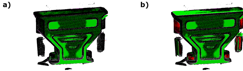
Figure 29: Geometric primitives extraction with a) mesh analysis and b) curvature analysis of Outlet .
