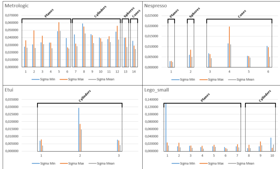
Figure 30: Noise in submesh minimum (blue, left), maximum (orange, middle) and mean (grey, right) curvature distributions. Each position on horizontal axis represents a different submesh, and vertical axis shows the corresponding standard deviation values.
