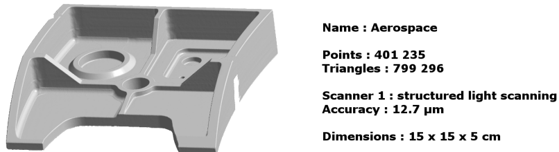
Figure 20: Initial mesh from Scanner 1: Aerospace .
