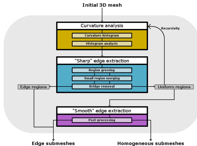
Figure 11: Segmentation overview based on the proposed curvature analysis.
