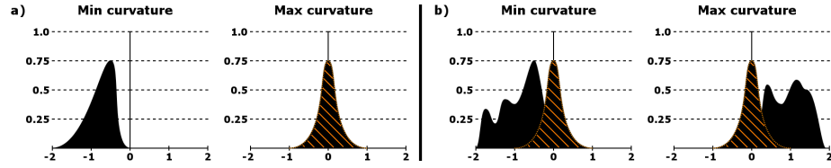
Figure 18: Principal curvature histograms: a) for a cone and b) for a developable surface. We can see in hatched orange a constant curvature which can be analyzed.
