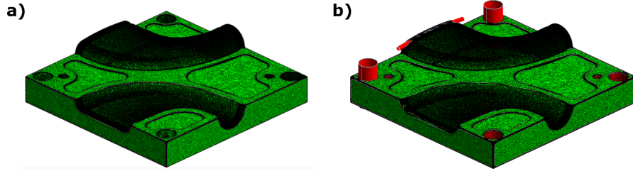
Figure 28: Geometric primitives extraction with a) mesh analysis and b) curvature analysis of Moldy .
