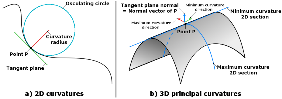
Figure 1: Curvature representation on: a) 2D curves and b) 3D surfaces.
