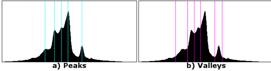
Figure 9: Histogram: a) peaks and b) valleys.
