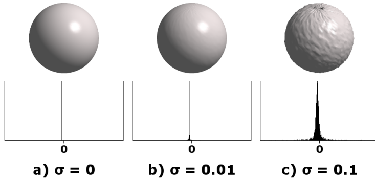
Figure 5: Spheres of radius r = 10 with gaussian noise and their corresponding mean curvature histogram: a) original sphere, b) \sigma = 0.01 , c) \sigma = 0.1 .
