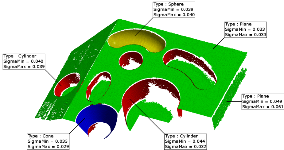
Figure 31: Primitive type detection and noise evaluation on Metrologic .
