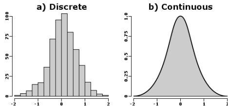
Figure 2: a) Discrete and b) Continuous distribution samples.
