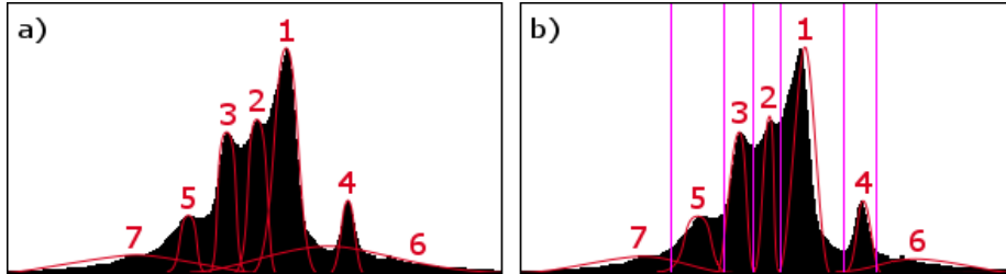
Figure 10: a) Gaussian Mixture Model of a histogram, b) Starting models with peak and valley detection.
