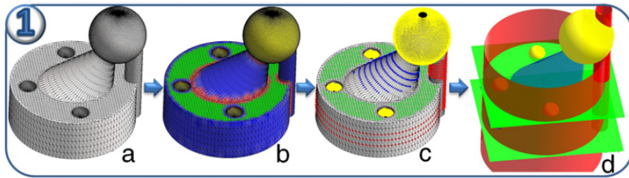
Figure 4: a) Original 3D mesh, b) Curvature: planar (green), spherical (yellow), convex (blue) and concave (red), c) Point areas, d) Extracted primitives [2].
