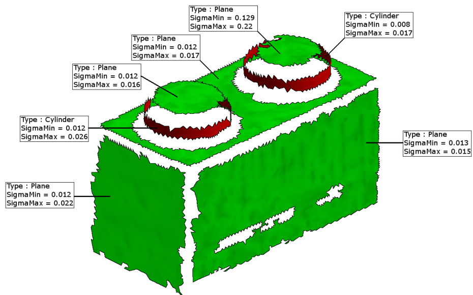
Figure 33: Primitive type detection and noise evaluation on Lego_small .
