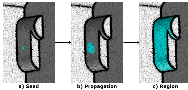
Figure 14: Region growing algorithm.
