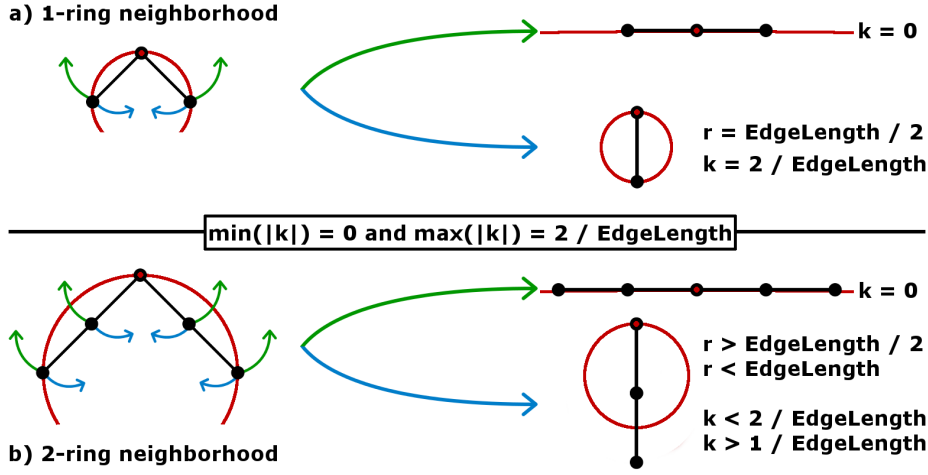
Figure 7: Minimum and maximum possible for absolute curvature values.
