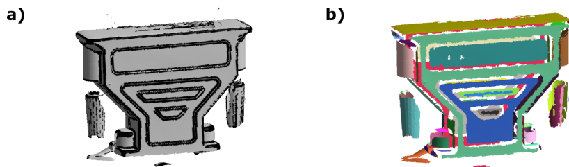
Figure 25: a) Edge extraction and b) Segmentation of Outlet .
