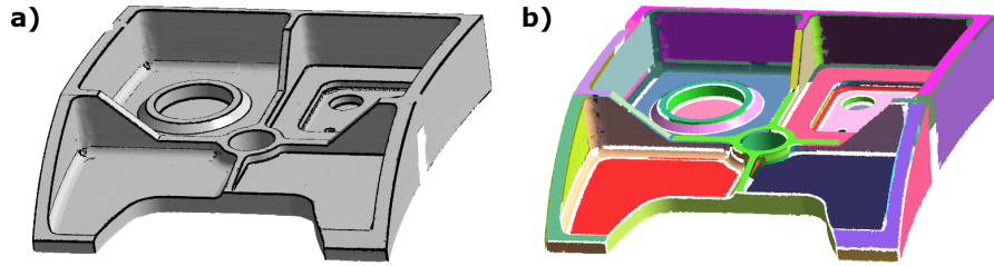
Figure 23: a) Edge extraction and b) Segmentation of Aerospace .
