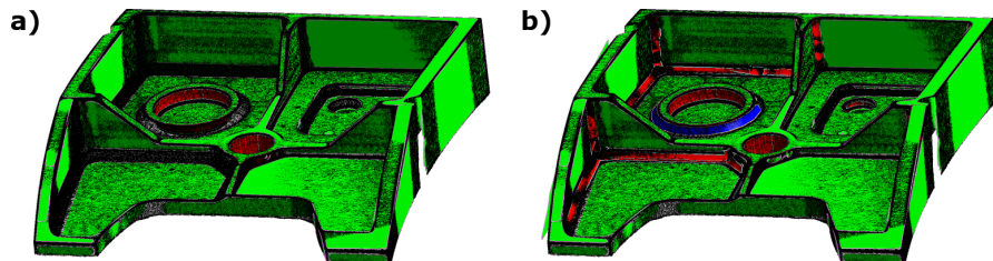
Figure 27: Geometric primitives extraction with a) mesh analysis and b) curvature analysis of Aerospace .
