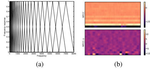
Fig. 4: Mel filterbank (a) and MFCC decomposition (b)
