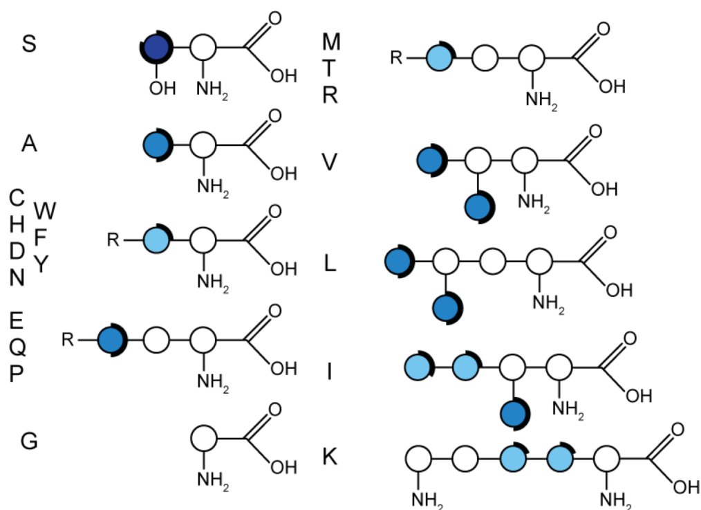
Fig. 8. Schematic representation of 1 H dilution by inverse fractional deuteration, based on biosynthetic pathway analysis and experimental data on expression in E. coli BL21(DE3) cells reported by Medeiros-Silva et al. [39]. The degree of 2 H incorporation is illustrated by black rings of growing angular width and blue circles of increasing intensity: 0 to 10% (white), 11 to 30% (light blue), 31 to 50% (medium blue), more than 51% (dark blue).
