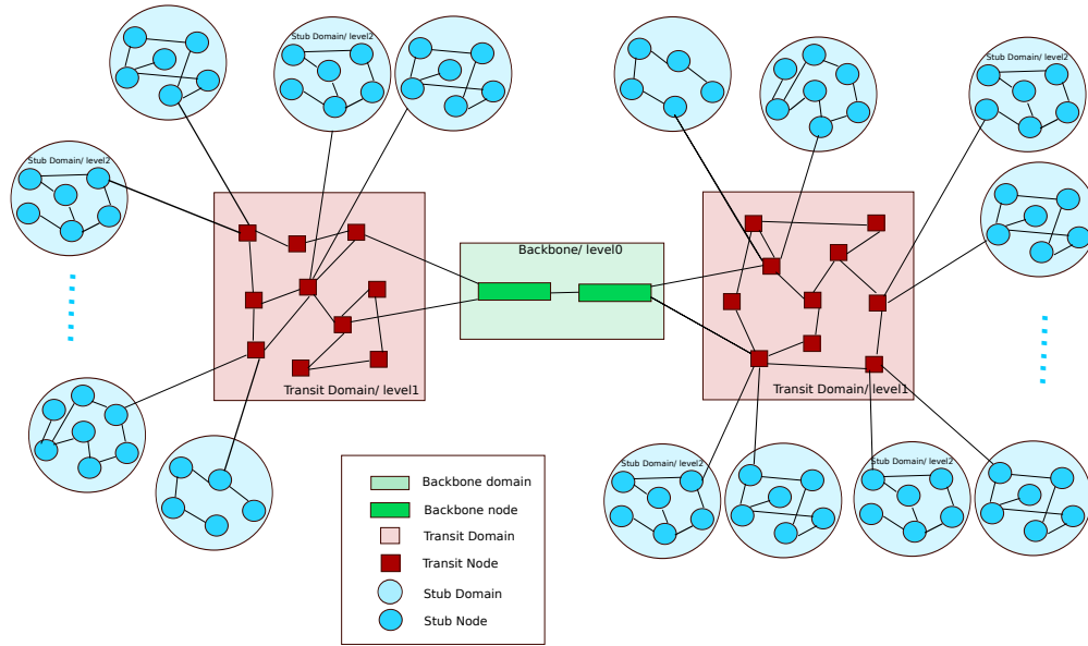
Fig. 3. Transit-Stub topology
