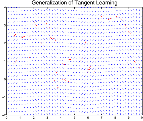
Figure 1: Task 1 2-D data with 1-D sinusoidal manifolds: the method indeed captures the tangent planes. The small segments are the estimated tangent planes. Red points are training examples.
