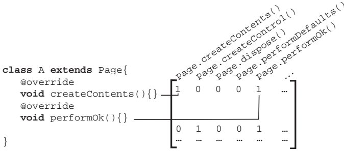
Fig. 3. Mapping Code to a Binary Space to Mine Extension Scenarios with LCA
