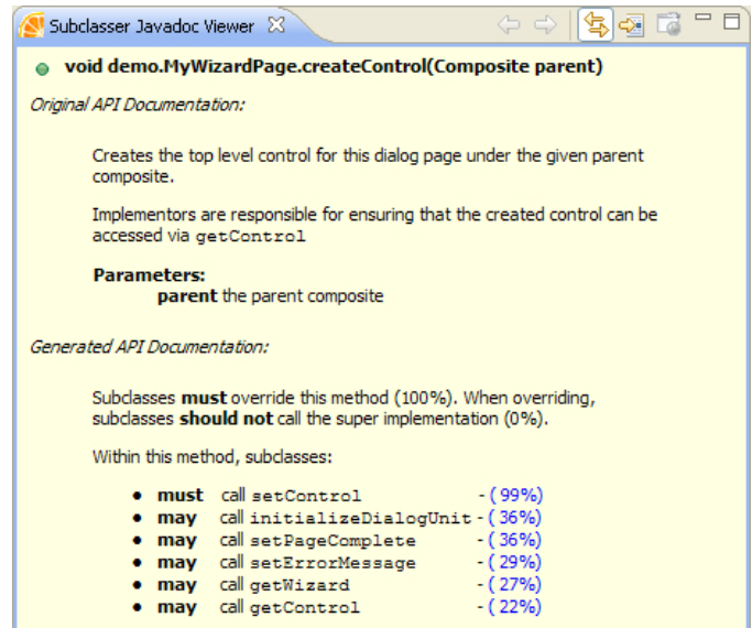
Fig. 5. Method-level API Documentation Extended with Automatically Mined Subclassing Directives.
