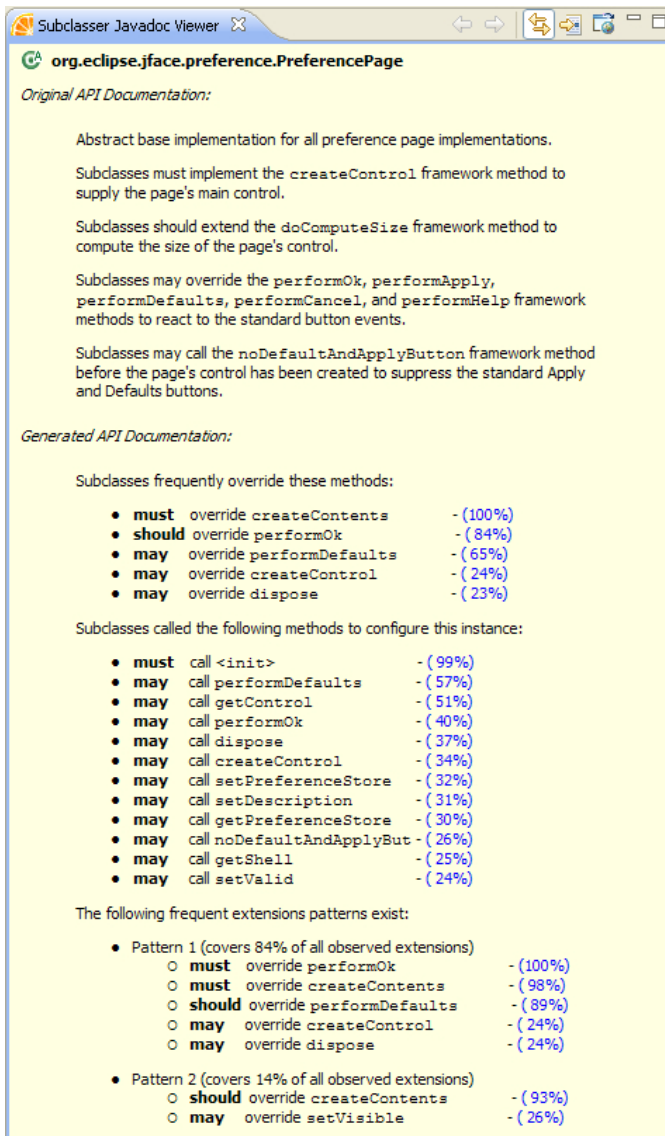
Fig. 4. Class-level API Documentation Extended with Automatically Mined Subclassing Directives.
