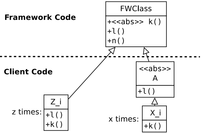
Fig. 2. An Example to Assess the Correctness of the Metric ovLikelihood
