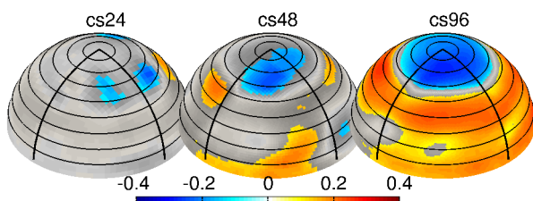
Fig. 10 Correlation between yearly Sea Level Pressure and the yearly MOC index 2 yr later (i.e. when the most significant correlations are found). Regions that are not statistically significant at the 5% level are grey shaded. The thin black contours mark latitude circles every 10° from 10°N to 80°N, and the thick orthogonal black lines the boundaries of the small basin
