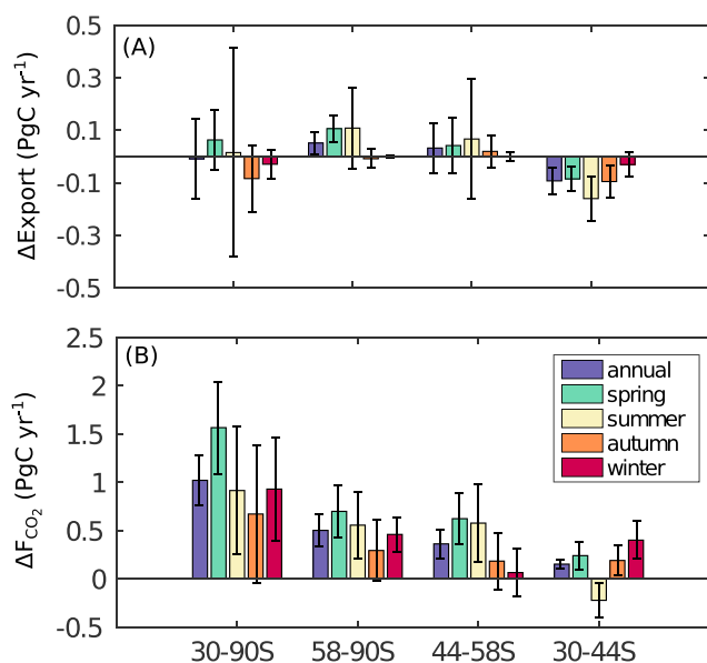
Figure 2. (a) \Delta Export production and (b) \Delta F_{\text{CO}_2} , both in units of \text{PgC yr}^{-1} , calculated as the average for period 2081–2100 minus the average for 2012–2031. Bars depict the multimodel mean, and error bars denote 1 standard deviation. If the error bar includes zero, the change is not significant.
