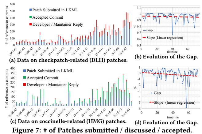
Figure 7: # of Patches submitted / discussed / accepted.
