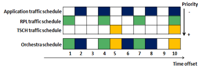
Fig. 1. Orchestra slotframes illustration (the slotframes lengths are 2, 3 and 5 corresponding to the application, routing and MAC slotframes respectively).
