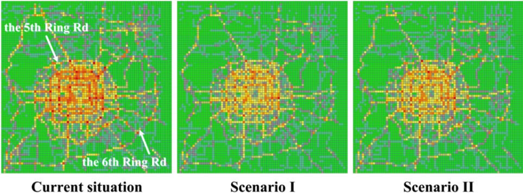
Figure 6. The gridding emission display of the 2 LEZ policy scenarios (1 km × 1 km) (CO is taken for example here).
