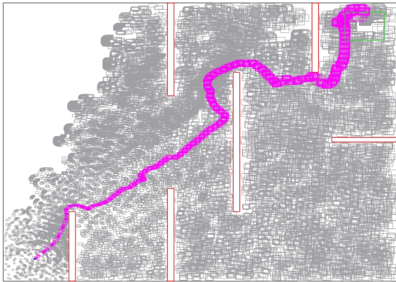
Figure 1: A BoxRRT* solution with [\mathbf{s}_{\text{init}}] the blue box and [\mathbf{s}_{\text{goal}}] the green one while the obstacles are in red: CPU = 745 [s], the number of vertices and the planned path length are 96 and 105 [cm], respectively, while the total number of vertices is 13655.
