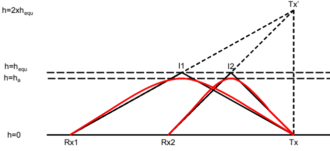
Fig. 2. Geometry of the HF localization principle considering uniform single layer ionosphere.
