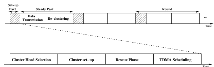
Fig. 1. Operating diagram of protocol cited in [11].
