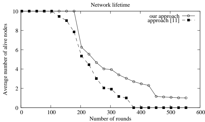
Fig. 4. Network lifetime.
