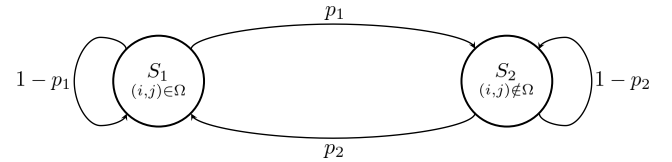
Figure 6. State diagram for the Markovian sampling model.
