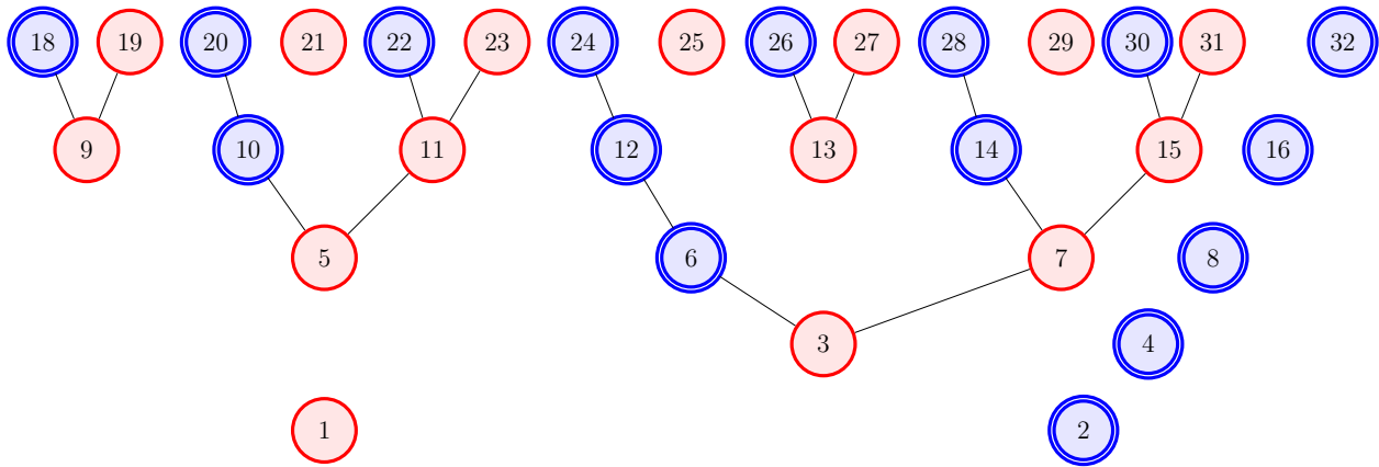
Figure 1. Binary tree
