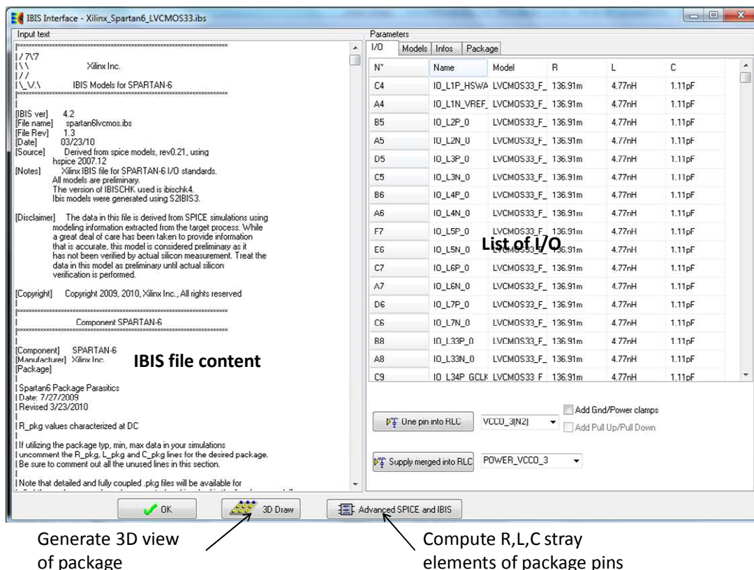
Figure 3- 30: Loading an IBIS file in the IBIS interface (examples\ibis\ Xilinx_Spartan6_LVCMOS33.ibs)
