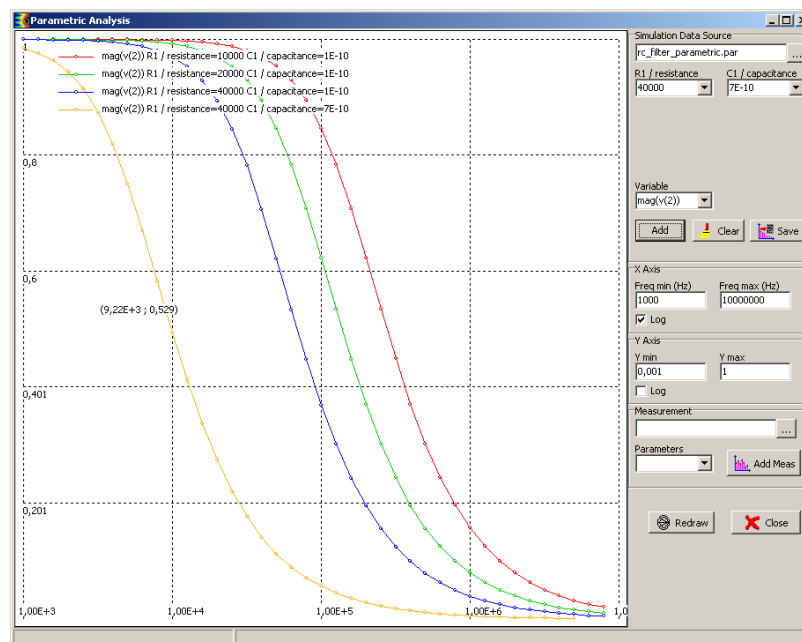
Figure 4- 30: Plot of the results of Parametric analysis (examples\misc\rc_filter_parametric.par)
