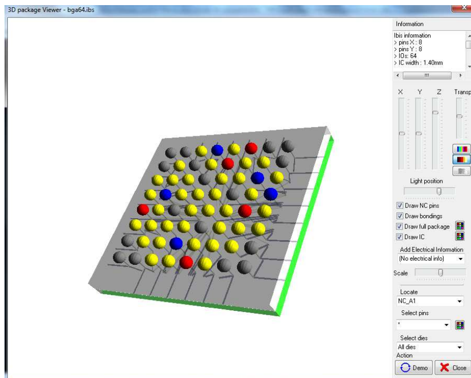
Figure 4- 35: the 3D-package viewer (examples\ibis\bga64.ibs)
