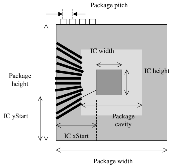
Figure 3- 33 : Main parameters required for an estimation of the package R,L,C model
