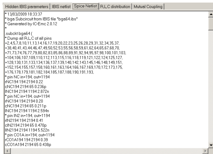
Figure 3- 82 : SPICE sub-circuit corresponding to the electric description of R,L and C (examples\ibis\BGA64.ibs)
