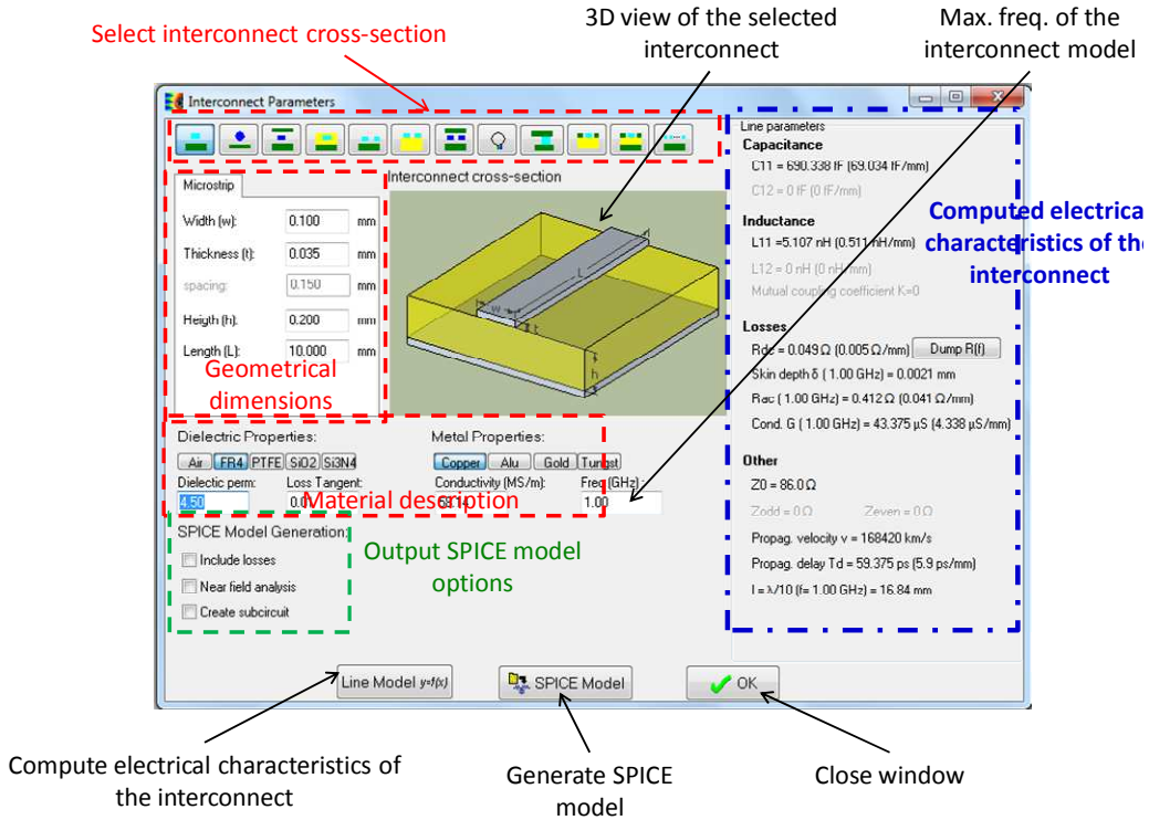
Figure 4- 39: Interconnect R,L,C model based on physical dimensions
