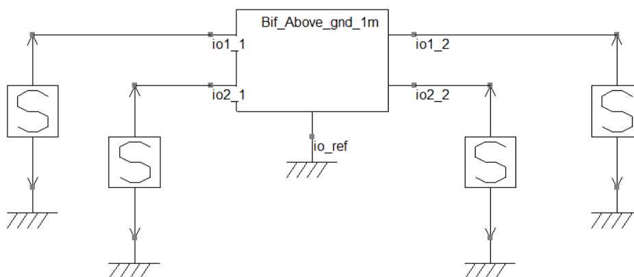
Figure 3- 74: S parameter simulation of a bifilar pair cable (\\Examples\\basic\\Cables\\Bif_above_gnd_1m.sch)
