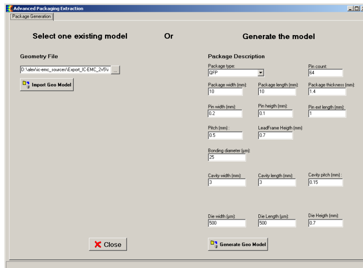
Figure 4- 36: Definition of package model, generation of .geo file
