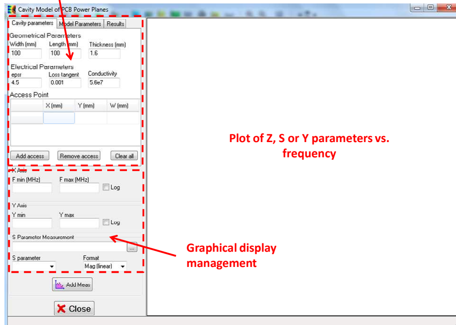
Figure 4- 41: Configuration of cavity dimensions and port placement
