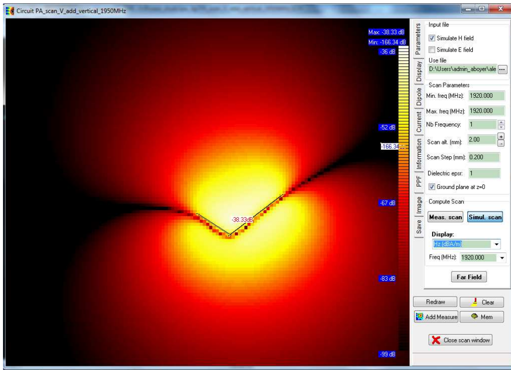
Figure 3- 62: Simulation of the vertical components of the magnetic field Hz simulated at 1920 MHz (Scan_Hx_PA_1950_1_5mm\PA_scan_V_add_vertical_1950MHz.sch)
