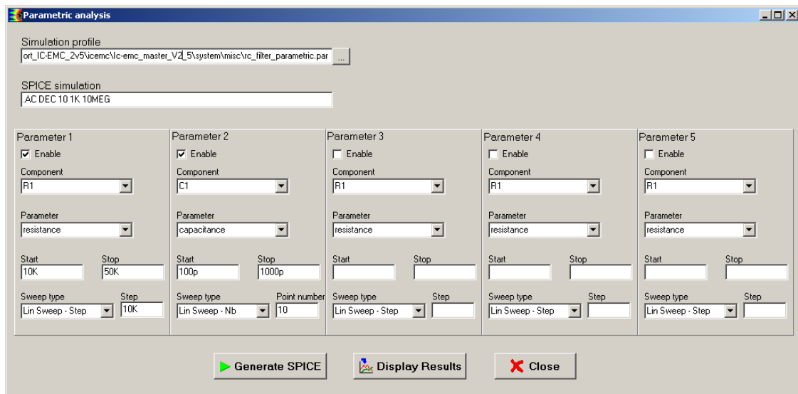
Figure 4- 29: Parametric analysis configuration interface (examples\misc\rc_filter_parametric.sch and examples\misc\rc_filter_parametric.par)
