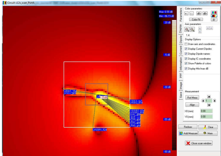
Figure 4- 21: The near-field scan user's interface (case_study\12x\12x_scan_portA.sch)
