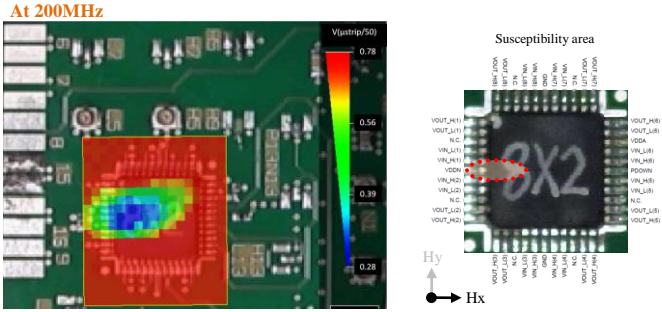
Fig 15. Hx Near-field immunity level at 200MHz
