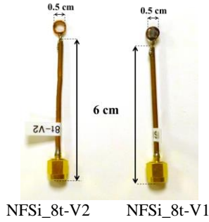
Fig 2. Dimensions of the tested near-field injection probe
