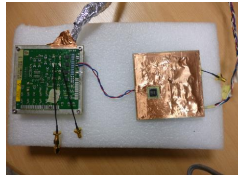
Fig 17. ARINC board modified for TEM measurement
