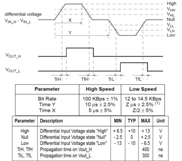
Fig 8. Transfer function diagram
