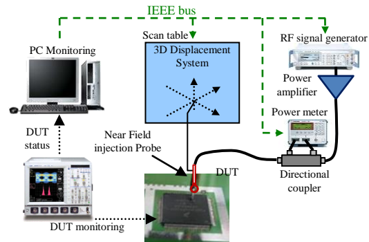
Fig 1. Test bench description
