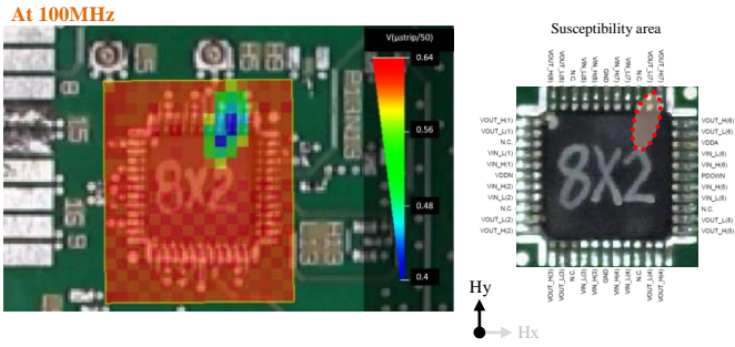
Fig 14. Hy Near-field immunity level at 100MHz
