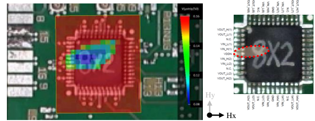
Fig 12. Hx Near-field immunity level (3MHz-10MHz)
