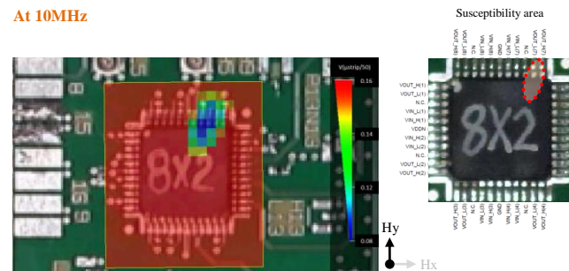
Fig 13. Hy Near-field immunity level (2MHz-10MHz)
