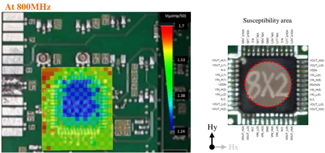
Fig 16. Hy Near-field immunity level at 800MHz
