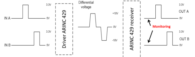
Fig 9. Encoding and decoding principle
