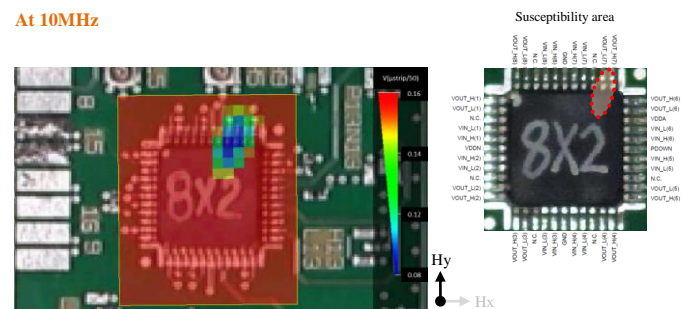
Fig 13. Hy Near-field immunity level (2MHz-10MHz)
