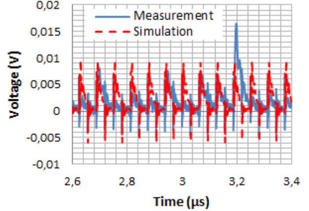
Fig. 9. Comparison between the measured and simulated external voltage using a 1\ \Omega probe in the time domain of the 7-bits counter configuration using the deterministic approach
