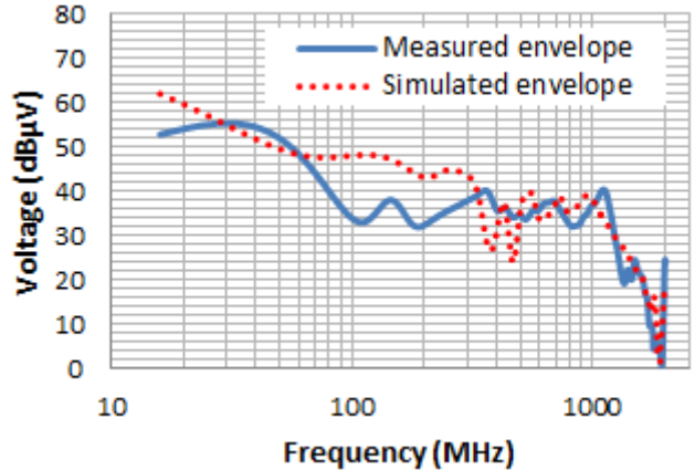
Fig. 10. Comparison between the measured and simulated external voltage using a 1 \Omega probe in the frequency domain of the 7-bits counter using the deterministic approach
