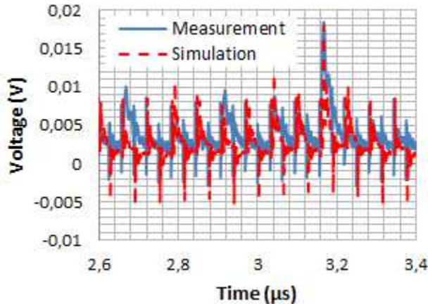
Fig. 11. Comparison between the measured and simulated external voltage using a 1\ \Omega probe in the time domain of the 7-bits counter using the random approach
