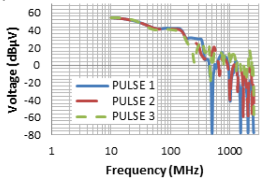
Fig. 2. Comparison between the simulations using the different shapes of IA with a 1 \Omega probe
