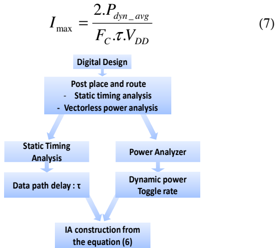
Fig. 3. Construction workflow of the Internal Activity block for FPGA circuit
