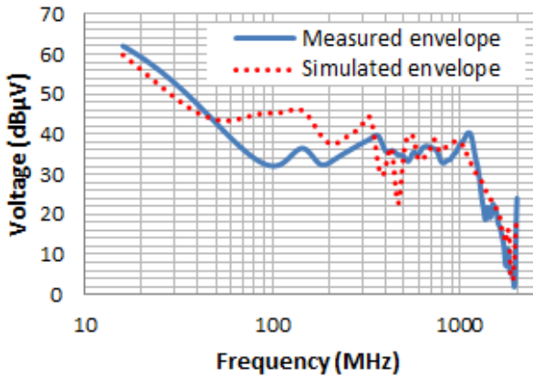
Fig. 8. Comparison between the measured and simulated external voltage using a 1 \Omega probe in the frequency domain of the delay line configuration
