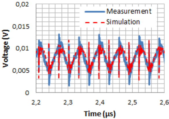
Fig. 7. Comparison between the measured and simulated external voltage using a 1 \Omega probe in the time domain generated by the delay line configuration
