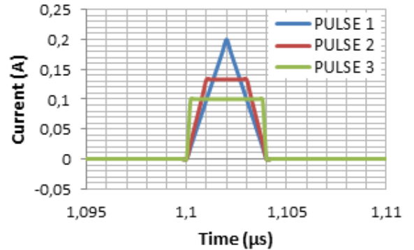
Fig. 1. Three basic pulsed waveforms to model the dynamic current consumption of a circuit
