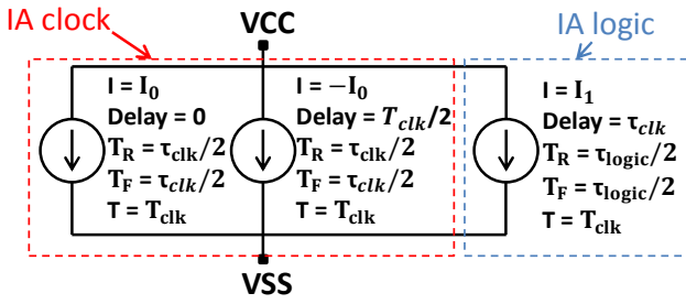
Fig. 6. Internal Activity of the core block
