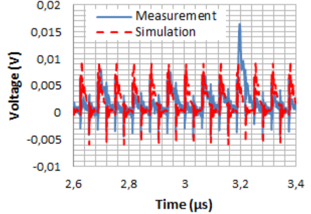
Fig. 9. Comparison between the measured and simulated external voltage using a 1 \Omega probe in the time domain of the 7-bits counter configuration using the deterministic approach
