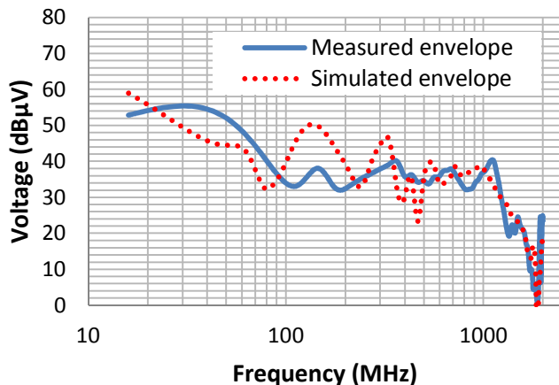
Fig. 12. Comparison between the measured and simulated external voltage using a 1\ \Omega probe in the frequency domain of the 7-bits counter using the random approach
