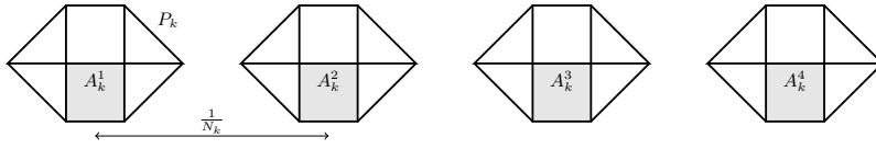
Figure 2. The function \beta_k is supported on the union of the N_k equispaced copies of P_k , while the function u_k is supported on the grey region given by \bigcup_{j=1}^{N_k} A_k^j .
