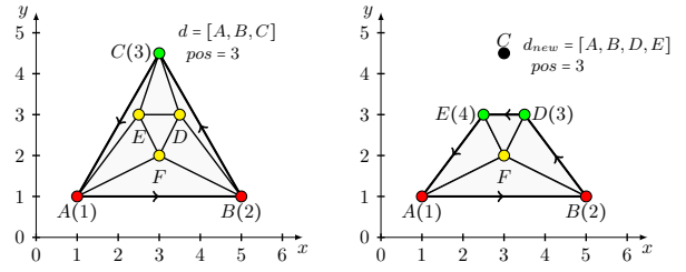
Figure 4: DELAUNAYENUM extreme point deletion.
