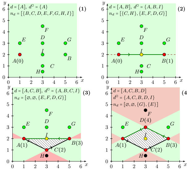
Figure 5: EXTREMEPOINTSENUM algorithm step-by-step enumeration.
