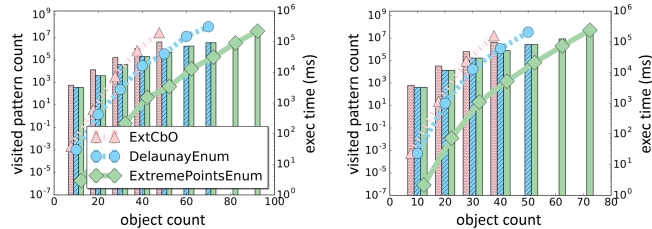
Figure 6: Polygon pattern enumeration performance comparison. IRIS sepal-length \times sepal-width (left). IRIS petal-length \times petal-width (right).
