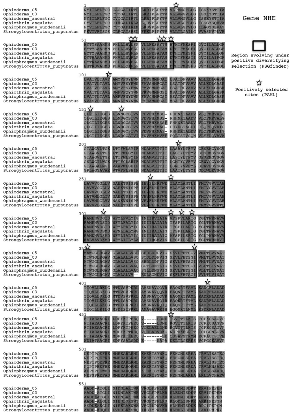
Fig. 3 NHE protein alignment including Ophioderma longicauda C3 and C5, as well as outgroups Ophiothrix angulata (brittle star), Ophiophragmus wurdemanii (brittle star) and Strongylocentrotus purpuratus (sea urchin). Ancestral sequence reconstruction of Ophioderma was performed with PAML version 4.8. The region evolving under positive selection detected by PSGfinder and the positively selected sites detected by PAML are displayed. The alignment highlights that positive diversifying selection occurred in the brooding species Ophioderma longicauda C5. Levels of grey correspond to different amino acid families.
