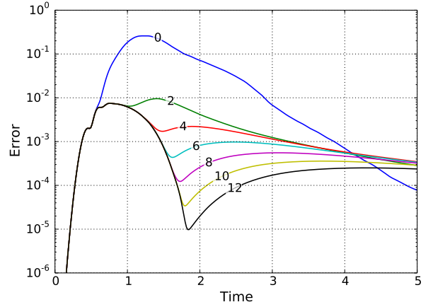
Figure 1: Error with HABCs having N additional fields ( N = 0, 2, \dots, 12 ). The main spherical wavefront is travelling in \Omega when t \in [0, 2] .
