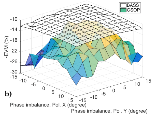
Fig. 4. Average EVM surfaces as a function of the a) gain imbalance and b) phase imbalance with 16-QAM modulations. Normalized residual CFO is set to 10^{-5} .
