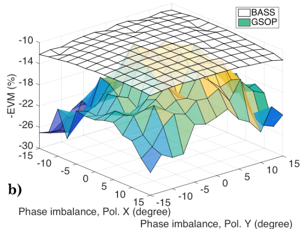
Fig. 4. Average EVM surfaces as a function of the a) gain imbalance and b) phase imbalance with 16-QAM modulations. Normalized residual CFO is set to 10^{-5} .
