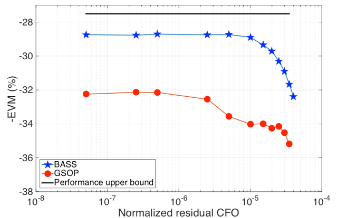
Fig. 6. Average EVM as a function of the normalized residual CFO with 4-QAM modulations. The sets of gain/ phase imbalance values of polarizations X and Y are 1.2/30^\circ and 1.1/30^\circ , respectively.
