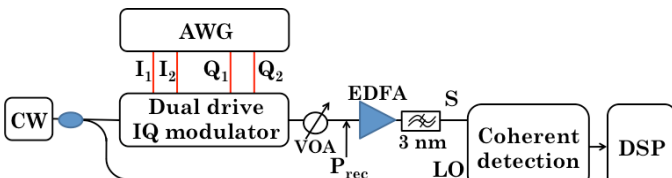
Fig. 8. Experimental setup for the validation of the Tx IQ imbalance compensation.
