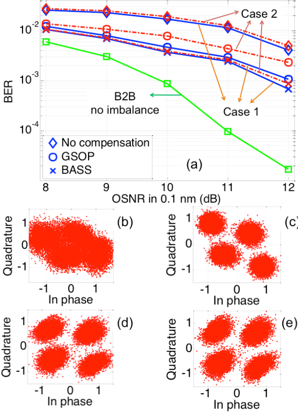
Fig. 9. (a) Evolution of the BER of a 10-Gbaud 4-QAM signal as a function of OSNR in the presence of 30^\circ phase imbalance (Solid lines: case 1; dash-dotted lines: case 2). Examples of 4-QAM constellations at 10-dB OSNR in the cases of (b) Raw data; (c) w/o IQ imbalance compensation; (d) w/ GSOP (case 2); (e) w/ BASS (case 2).
