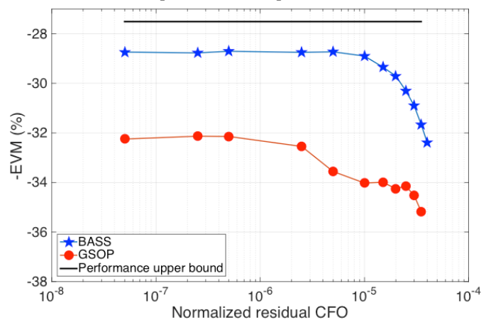
Fig. 6. Average EVM as a function of the normalized residual CFO with 4-QAM modulations. The sets of gain/ phase imbalance values of polarizations X and Y are 1.2/ 30^\circ and 1.1/ 30^\circ , respectively.
