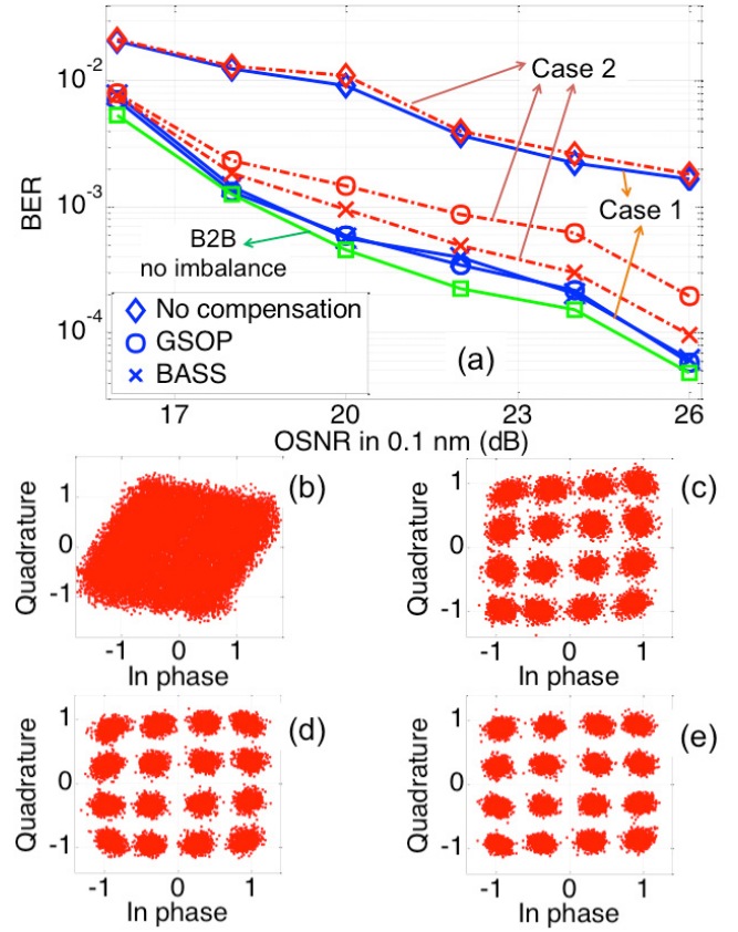
Fig. 10. (a) Evolution of the BER of a 10-Gbaud 16-QAM signal as a function of OSNR in the presence of 10^\circ phase imbalance (Solid lines: case 1; dash-dotted lines: case 2). Examples of 16-QAM constellations at a 26-dB OSNR in the cases of (b) Raw data; (c) w/o IQ imbalance compensation; (d) w/ GSOP (case 2); (e) w/ BASS (case 2).
