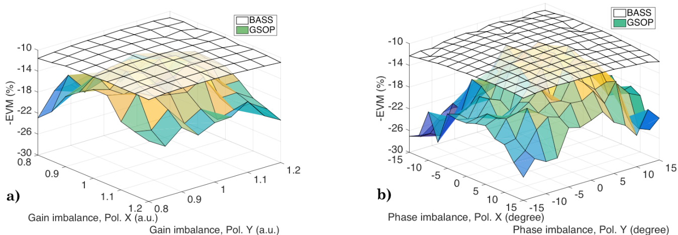
Fig. 4. Average EVM surfaces as a function of the a) gain imbalance and b) phase imbalance with 16-QAM modulations. Normalized residual CFO is set to 10^{-5} .
