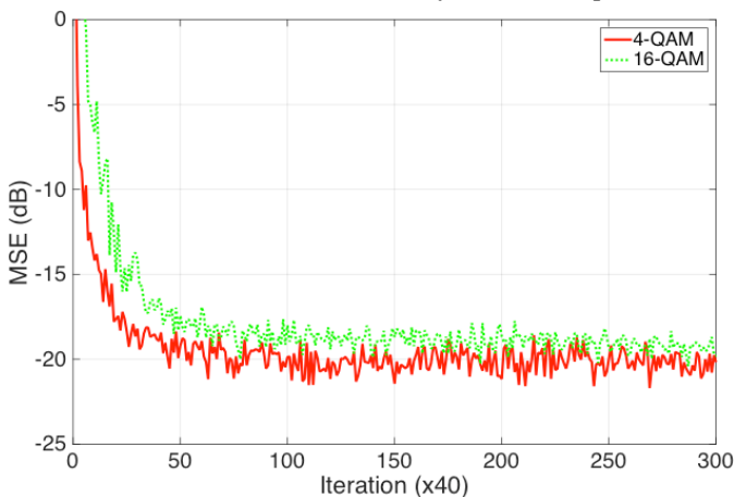
Fig. 5. Convergence speed of adaptive algorithm using the BASS algorithm for 4- and 16-QAM modulations. MSE calculation is averaged over two polarizations and over 100 simulation runs.
