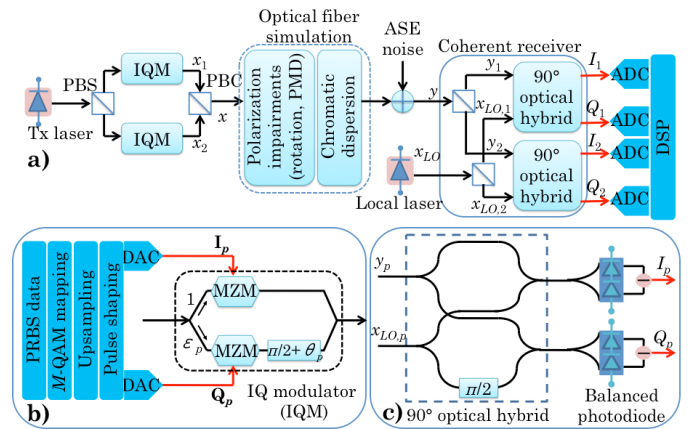
Fig. 1. a) Block diagram of the dual polarization M -QAM coherent transmission system under the impacts of Tx IQ imbalance, CFO, CD and polarization multiplexing induced effects. b) Tx electrical signal generation and IQ modulator structure with IQ imbalance. c) 90° optical hybrid structure. PBS: polarization beam splitter, PBC: polarization beam combiner.
