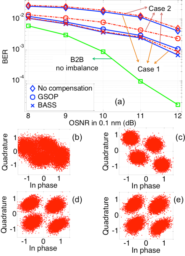
Fig. 9. (a) Evolution of the BER of a 10-Gbaud 4-QAM signal as a function of OSNR in the presence of 30^\circ phase imbalance (Solid lines: case 1; dash-dotted lines: case 2). Examples of 4-QAM constellations at 10-dB OSNR in the cases of (b) Raw data; (c) w/o IQ imbalance compensation; (d) w/ GSOP (case 2); (e) w/ BASS (case 2).
