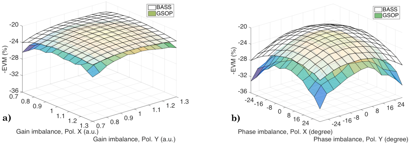
Fig. 3. Average EVM surfaces as a function of the a) gain imbalance and b) phase imbalance with 4-QAM modulations. Normalized residual CFO is set to 10^{-5} .
