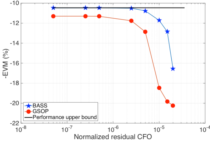
Fig. 7. Average EVM as a function of the normalized residual CFO with 16-QAM modulations. The sets of gain/phase imbalance values of polarizations X and Y are 1.1/10^\circ and 1.05/10^\circ , respectively.
