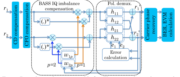
Fig. 2. Digital signal processing blocks. The received complex signal is r_p = I_p + jQ_p .
