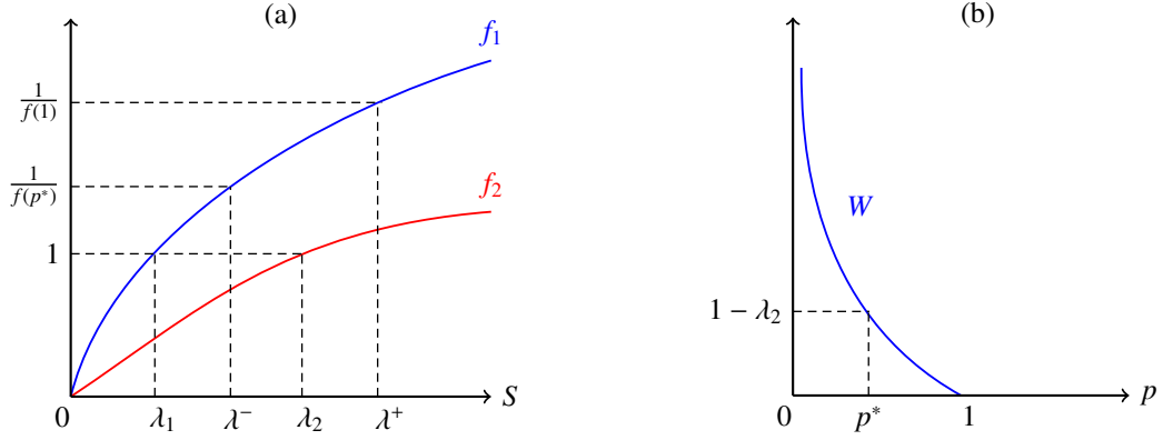
Figure 1: Illustrative graphs of functions (a): f_1 and f_2 and definitions of break-even concentrations \lambda_1 , \lambda_2 , \lambda^+ and \lambda^- which are given by (6) and (8), respectively; (b): W with the unique positive solution p^* of equation W(p) = 1 - \lambda_2 , when \lambda_2 < 1 .
