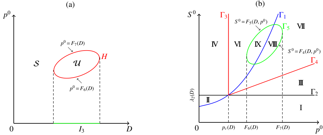
Figure 5: (a): The curve H defined by (58) separates the plane (D, p^0) in two regions U and S so that if (D, p^0) \in S , the positive equilibrium E_c is stable for any S^0 . The condition (D, p^0) \in U is necessary of E_c to be unstable. (b): The construction of the curve \Gamma_5 when D is fixed in the subset I_3 and F_6(D) \leq p^0 \leq F_7(D) . The figure illustrate a case where \Gamma_5 intersects \Gamma_1 , so that both regions VIII and IX exist.
