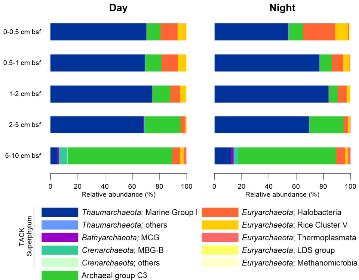
Figure 4. Distribution of archaeal 16S rRNA transcripts. The relative abundance of the 16S rRNA transcripts and the affiliation of the total archaeal operational taxonomic units (OTUs 97%) at the class level between the two Day and Night treatments among the five layers below the sediment surface (bsf).
