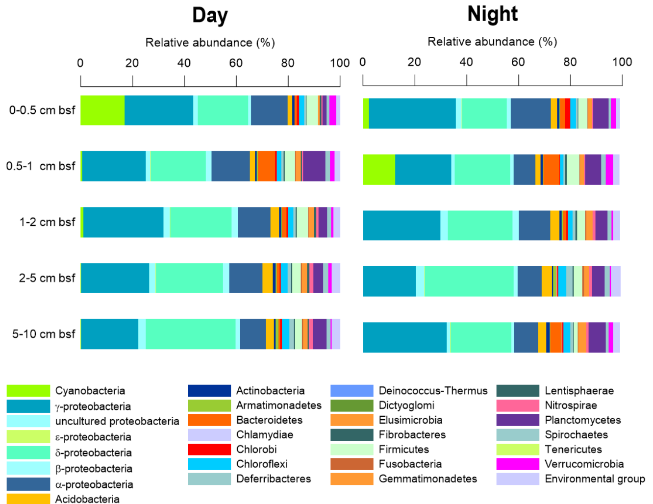
Figure 3. Distribution of bacterial 16S rRNA transcripts. The relative abundance of the 16S rRNA transcripts and the affiliation of the total bacterial operational taxonomic units (OTUs 97%) at the phylum level (except for Proteobacteria , class level) between the two Day and Night treatments among the five layers below the sediment surface (bsf). Environmental group contained BHI80-139, Candidate division OD1, Candidate division OP3, Candidate division TM7, Candidate division WS3, EM19, GOUTA4, Hyd24-12, JL-ETNP-Z39, LD1-PA38, NPL-UPA2, TA06 and TM6. Note that plastids originated from microalgae were removed from the dataset.
