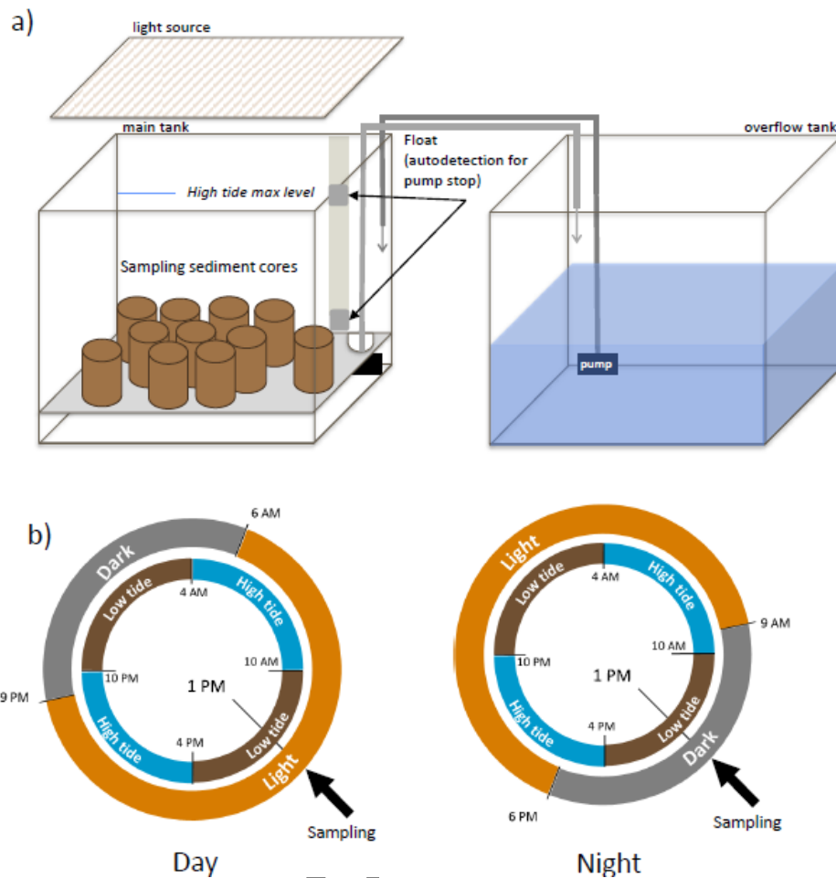
Figure 1. Schematic view of the experimental design. a) One mesocosm consisted of two tanks: a main and overflow tank, b) schedule for the Day and Night mesocosms.
