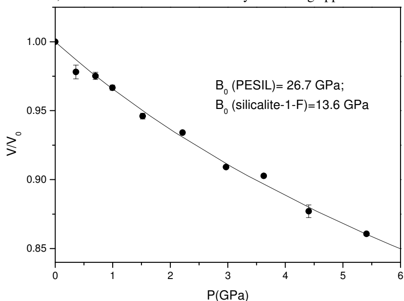
Figure 5. EOS of PESIL: relative volume data (dots) vs. P . A third order Birch-Murnagm EOS with a B_0 value of 26.7(2.0) GPa and the first derivative ( B_0' ) of 4 has been fitted to the experimental points.
