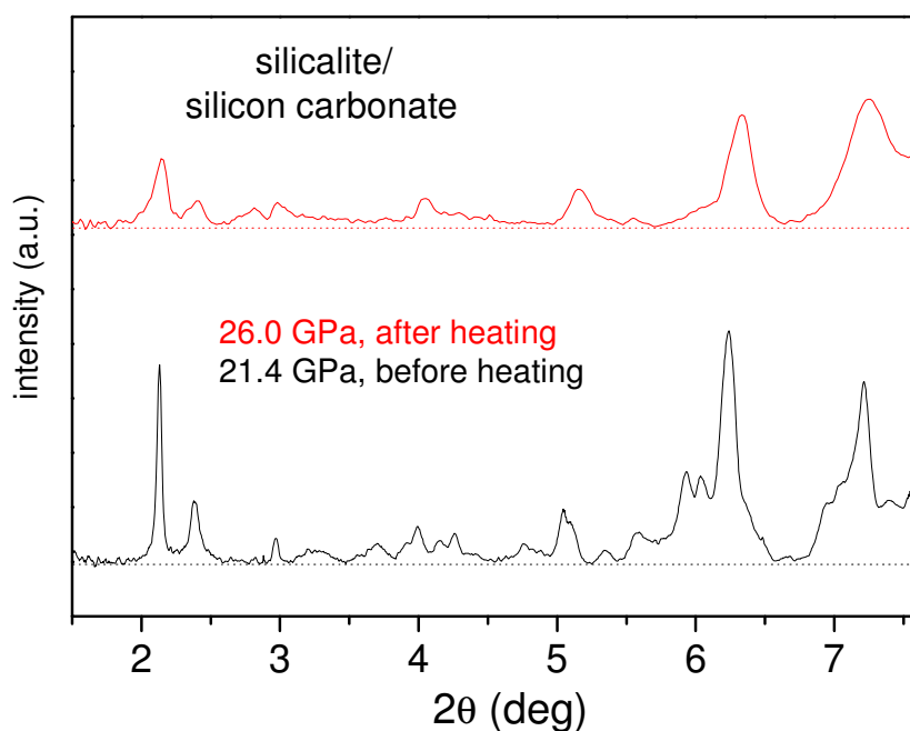
Figure 3. High pressure, synchrotron (ESRF-ID27, \lambda=0.3738 \text{ \AA} ) XRD patterns of a silicalite/CO 2 mixture before and after the heating to 723 K, showing the formation of a highly strained, disordered crystal. Sample thickness: about 20 \mu\text{m} . At angles higher than 7.5° the diffraction pattern is dominated by the peaks of bulk, molecular CO 2 .
