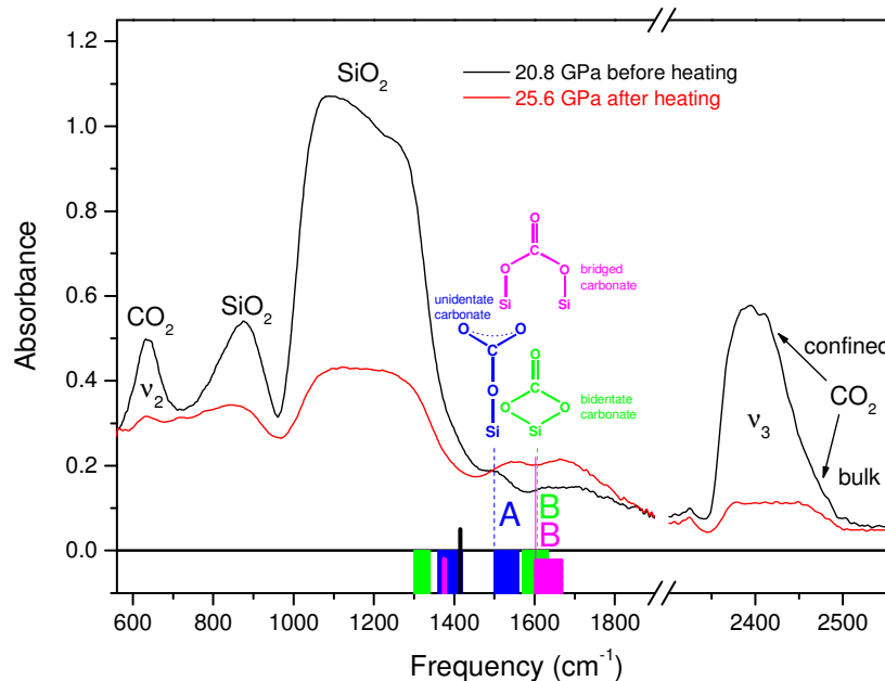
Figure 2. High pressure IR spectra before and after the heating to 740 K of a mixture of silicalite and CO 2 , showing the formation of silicon carbonate. The A and B peaks are assigned to unidentate (A), bidentate (B) and bridged (B) silicon carbonate species. Vertical black stick: frequency of the IR stretching mode of the free CO 3 ion. Bars: spectral ranges, at ambient pressure, of the split high and low frequency components of the IR stretching mode of the free CO 3 ion, as found in unidentate (blue), bidentate (green) and bridged (pink) carbonates, obtained from CO 2 adsorption on metal oxides and dissolution in silicate melts. Vertical lines: room pressure extrapolated frequencies of the A and B peaks.
