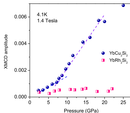
Figure 5. XMCD amplitude as a function of pressure.
