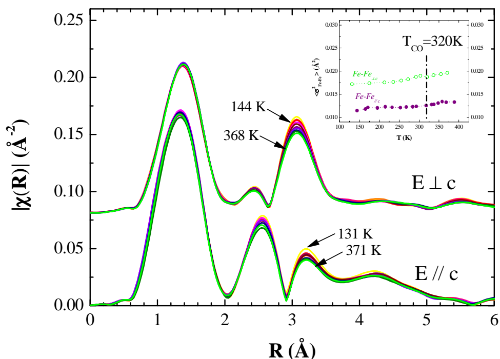
Figure 4. Temperature dependence of the moduli of the FTs of the k -weighted EXAFS signals at the Fe K-edge of \text{LuFe}_2\text{O}_4 for the two polarizations \mathbf{E} \perp \mathbf{c} and \mathbf{E} \parallel \mathbf{c} . Inset: Thermal dependence of the refined Debye-Waller factors ( \sigma^2 ) for the \text{Fe-Fe}_{\perp c} and \text{Fe-Fe}_{\parallel c} distances. The temperature of the CO transition is indicated.
