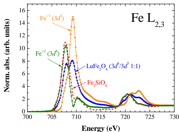
Figure 2. XANES spectra at the Fe L_{2,3} -edges of \text{LuFe}_2\text{O}_4 , \text{Fe}^{+3} ( \text{LuFeCoO}_4 ) and \text{Fe}^{+2} (deduced from the difference 2\mu_{\text{LuFe}_2\text{O}_4} - \mu_{\text{LuFeCoO}_4} ). The spectra of \text{Fe}_2\text{SiO}_4 with only \text{Fe}^{+2} taken from ref. [8] is also plotted for comparison.
