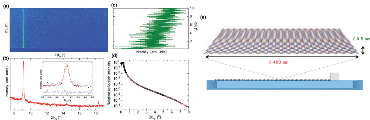
Fig. 4 (a) In situ grazing incidence X-ray diffraction reciprocal space map (diffracted intensity along 2\theta_{xy} (horizontal) and 2\theta_z (vertical) diffraction angles, \lambda = 1.549 \text{ \AA} , incidence angle, \alpha = 0.12^\circ ) of the NAFS-21 nanosheets collected at the air–liquid interface at a surface pressure, \pi = 5 \text{ mN m}^{-1} . (b) Integrated in-plane XRD profile (summed over the vertical diffraction angle, 2\theta_z range of 0\text{--}0.5^\circ ). The inset shows observed (solid circles) and fitted (red solid line) profiles in the vicinity of the (110) Bragg reflection. The lower blue solid line shows the difference profile. (c) Out-of-plane XRD profile obtained following integration of the XRD 2D map over the 2\theta_{xy} range of 9.08\text{--}9.17^\circ in the vicinity of the (110) Bragg reflection. (d) Observed (black circle) and fitted (two-layer model, red solid line) in situ X-ray reflectivity profile of the NAFS-21 nanosheets collected at the air–liquid interface at a surface pressure, \pi = 1 \text{ mN m}^{-1} . (e) Schematic illustration of the high aspect ratio NAFS-21 nanosheets (width >400 \text{ nm} , thickness <0.5 \text{ nm} ) assembled at the air–liquid interface.
