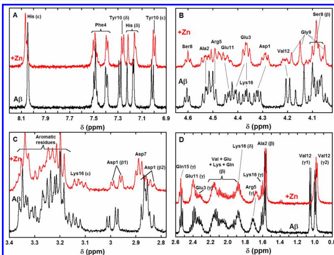
Figure 2. ^1\text{H} NMR spectra of A \beta (bottom black lines) and of A \beta in the presence of 0.9 equiv of Zn(II) (top red lines) in selected regions (A: aromatic, B: H \alpha , C: H \beta , D: H \beta and H \gamma , unless otherwise specified). [A \beta ] = 300 \mu\text{M} , [Zn(II)] = 270 \mu\text{M} in \text{d}_{11} -TRIS buffer 50 mM, pH = 7.4, T = 318 K, \nu = 500 MHz. \delta(\text{His6 H}\delta) > \delta(\text{His14 H}\delta) > \delta(\text{His13 H}\delta) . For the details of the amino acid residue nomenclature, see Scheme S1.
