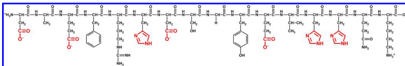
Scheme 1. A\beta Peptide in the Protonation State Predominant at pH 7.4 a
