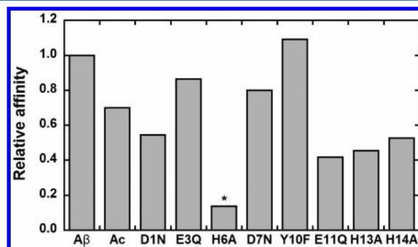
Figure 3. Zn(II) binding affinity values for the various modified peptides relative to A \beta . For the H6A mutant (*), the given value corresponds to a maximum value.
