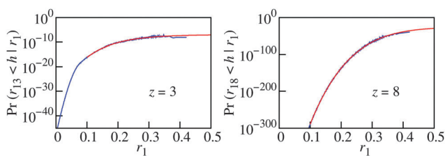
Fig. 5 Extrapolating the zero distance probability G_{1z}(h|r_1) (blue lines) using eqn (27) (red lines). G_{1z}(h|r_1) \equiv \Pr(r_{1z} < h | r_1) is the probability that a pore with radius r_1 will have exactly z contacts with real particles in a shell of width h . The data represent 39 combined fluidized bed packings (Q_150) with an average \phi of 0.585. The particle diameter is normalized to unity, the extrapolation is therefore to r_1 = 0.5 .
