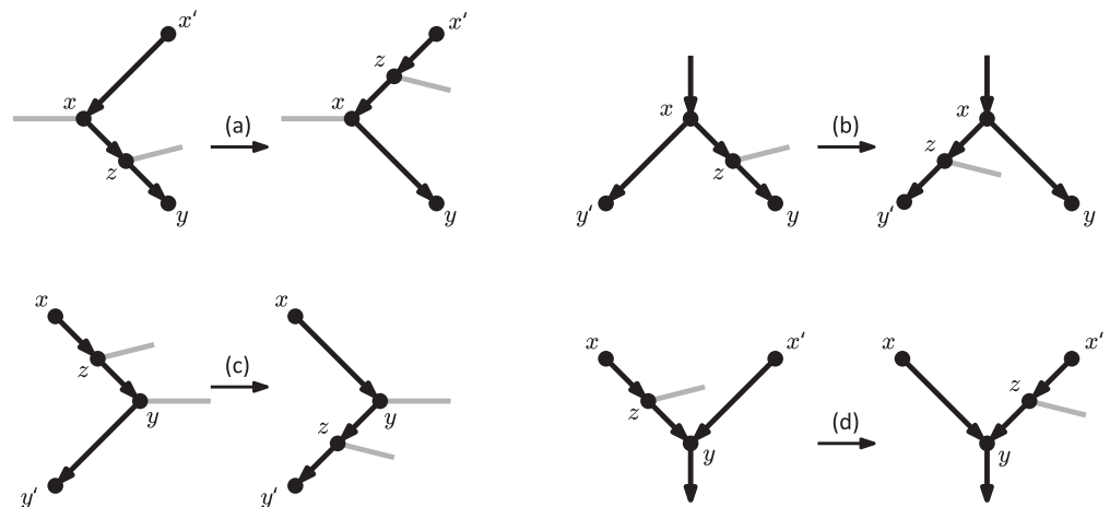
Fig 7. Illustration of \text{rSPR}_1 moves.
