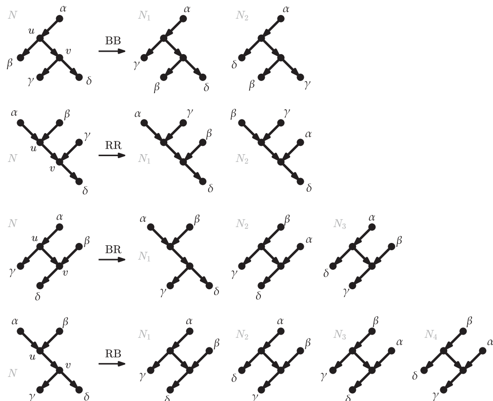
Fig 8. rNNI moves around the different types of internal arcs.
