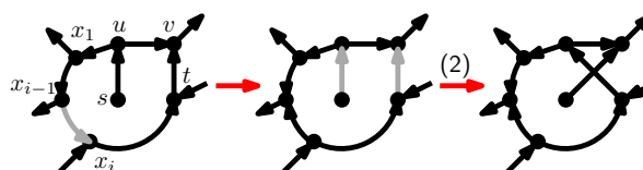
Figure S8. Avoiding directed cycles in Case (2) when t is a reticulation.
