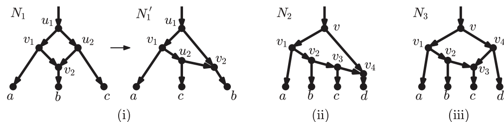
Fig 9. Reasons why the bound of Prop. 2 is not tight.
