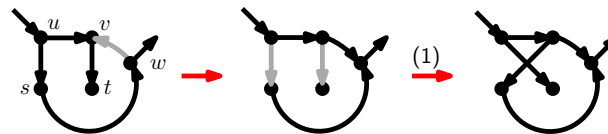
Figure S4. Avoiding directed cycles in Case (1) when w is a bifurcation. Note that the arc leaving w that does not point at v could point at t .
