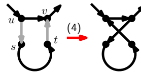
Figure S12. A cycle-creating rNNI move of type (4).
