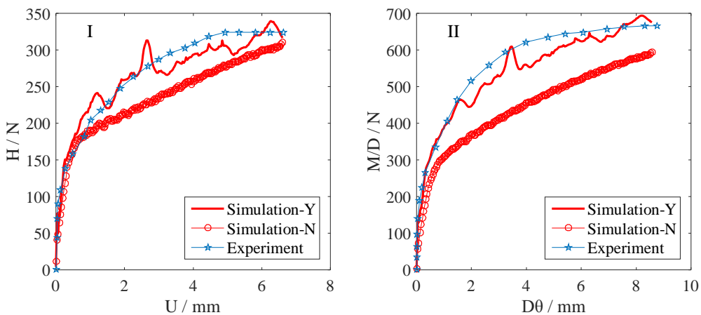
(b) M/DH=1.987
