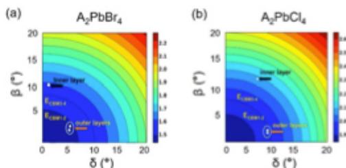
Figure 9. 2D color map of the electronic band gap variation including spin-orbit coupling with respect to octahedral distortions defined in Figure 4 for model systems \text{A}_2\text{PbBr}_4 and \text{A}_2\text{PbCl}_4 ( A = \text{Cs} ). Distortion angles of the inner and outer octahedral layers for \text{EA}_4\text{Pb}_3\text{Br}_{10} and \text{EA}_4\text{Pb}_3\text{Cl}_{10} are pointed to by the arrows in \text{A}_2\text{PbBr}_4 and \text{A}_2\text{PbCl}_4 respectively. ECBM1-2 and ECBM3-4 indicate the contour levels corresponding to their values from the band structure of Figure 7.
