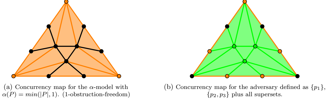
Figure 5: Examples of concurrency maps in two models of 3-process system, a color set to green corresponding to a concurrency value equal to 2, orange to 1, and black to 0. Note that p_1 is the vertex on the top.
