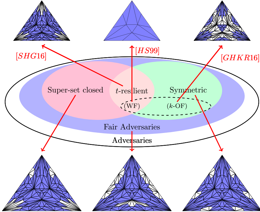
Figure 2: Earlier topological characterizations (wait-free [19], t -resilient [26], and k -obstruction-free [12]) and our contribution: affine tasks for all fair adversaries.
