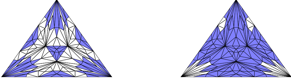
(a) Affine task for the \alpha -model with \alpha(P) = \min(|P|, 1) . (b) Affine task for the adversary defined as \{p_1\}, \{p_2, p_3\} plus all supersets. (1-obstruction-freedom)
