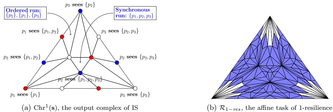
Figure 1: Standard chromatic subdivision and affine tasks.
