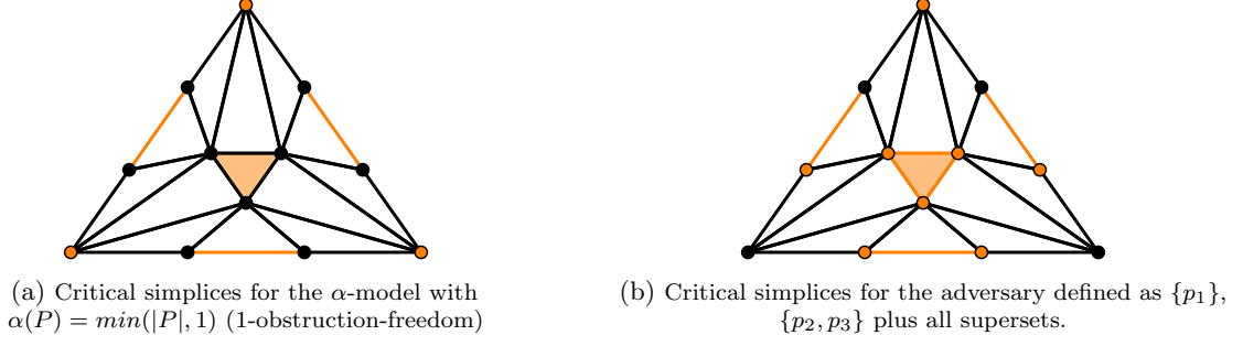
Figure 4: Critical simplices are displayed in orange (with p_1 associated to the vertex on the top).
