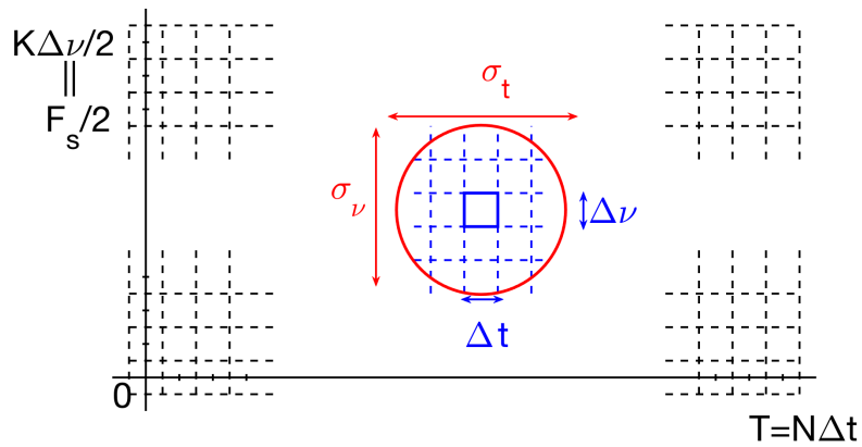
Figure 3: Illustration of the discrete time-frequency plane \{(n\Delta t, k\Delta\nu), 0 \leq n \leq N - 1, 0 \leq k \leq K/2\} . The resolution of the spectrogram is controlled by the analysis window's Gabor parameters (\sigma_t, \sigma_\nu) .
